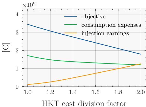
Figure 4: Evolution of the overall cost, the consumption from the grid and the injection earnings as a function of the decrease of the CAPEX and OPEX of HKT - system 2.1.
