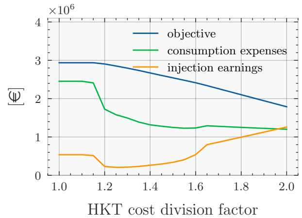
Figure 8: Evolution of the overall costs, the purchase of electricity from the grid, and the injection earnings as a function of the decrease of the overall yearly cost of HKT - system 2.2.
