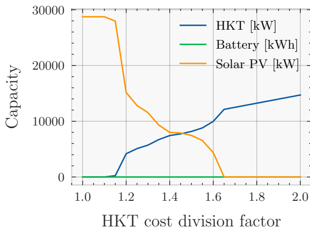
Figure 7: Evolution of the installed capacities of HKT, solar PV and battery storage as a function of the decrease of the CAPEX and OPEX of HKT - system 2.2.
