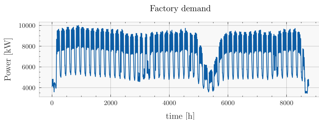
Figure 13: Electricity demand for subsystems 2.1 and 2.2.
