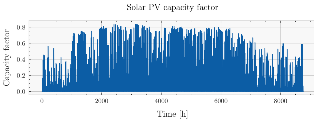
Figure 10: Capacity factor times series for solar PV production for the Paimpol-Bréhat location, obtained from the Renewable Ninja website, year 2019.
