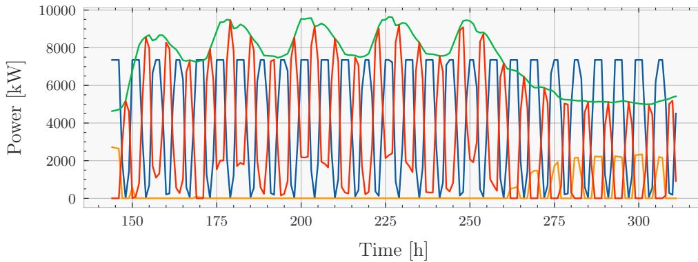
Figure 3: Graphical illustration of a typical behaviour of the system during a winter week showing the power produced by HKT in blue, the demand curve in green, the consumption from the grid in red and the injection into the grid in orange - system 2.1.
