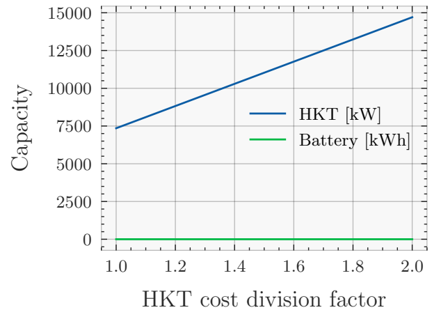
Figure 5: Evolution of the installed capacities for HKT and battery storage as a function of the HKT overall yearly costs decrease - system 2.1.
