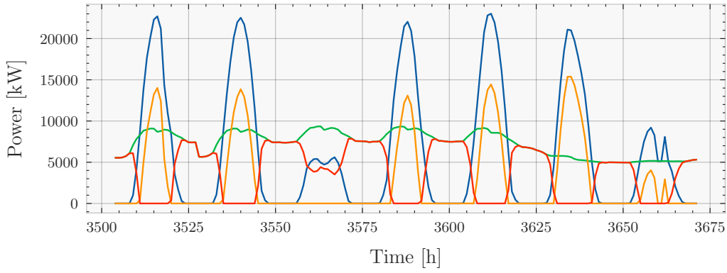
Figure 6: Graphical illustration of a typical behaviour of the system during a summer week showing the power produced by solar PV in blue, the demand curve in green, the injection into the grid in orange and the consumption from the grid in red - system 2.2.
